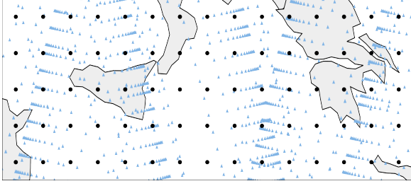
Figure 1: Location of satellite observations (blue \blacktriangle ) and grid points (gray \bullet ) for a single prediction step. The satellite paths used for reconstructing the observation locations are computed based on the orbital elements of METOP-B, METOP-C and NOAA 15 as measured by NORAD [22].
